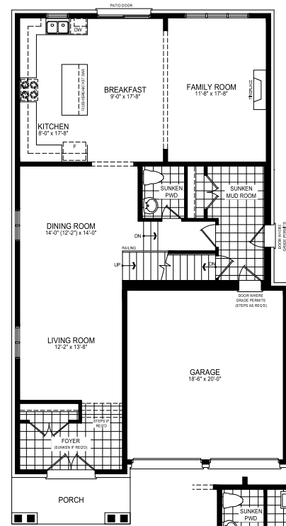
ELEV. A MAIN LEVEL
