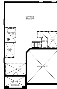
ELEV. A, B & C LOWER LEVEL
